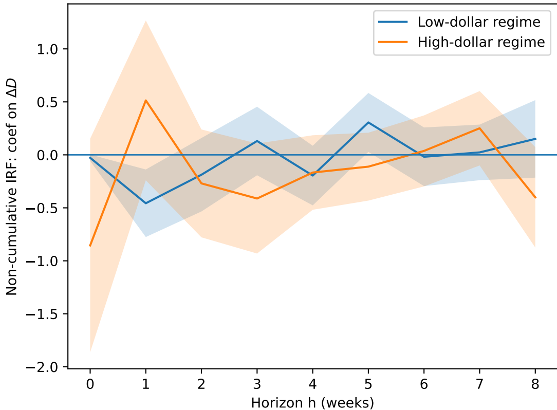
Regime-conditional local projections (non-cumulative, JPY basis 30Y)
